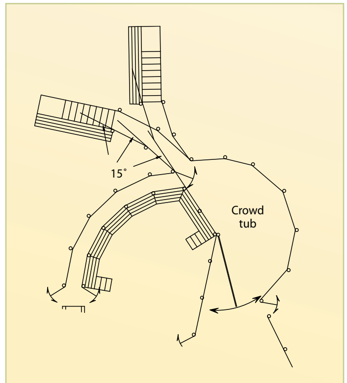
FIGURE 75. Loading alley and chute
