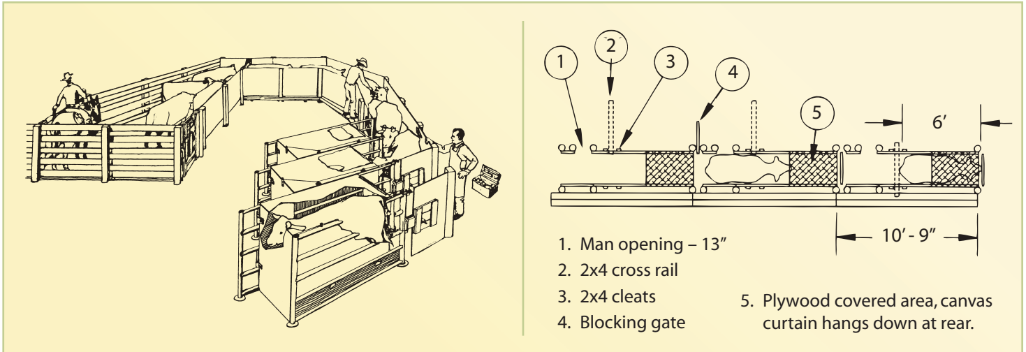
FIGURE 21. Two versions of a pregnancy testing and AI chute containing a “dark box” (Herringbone and Straight Alley).
