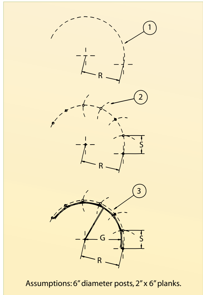
FIGURE 82. How to lay out a circular crowding tub
