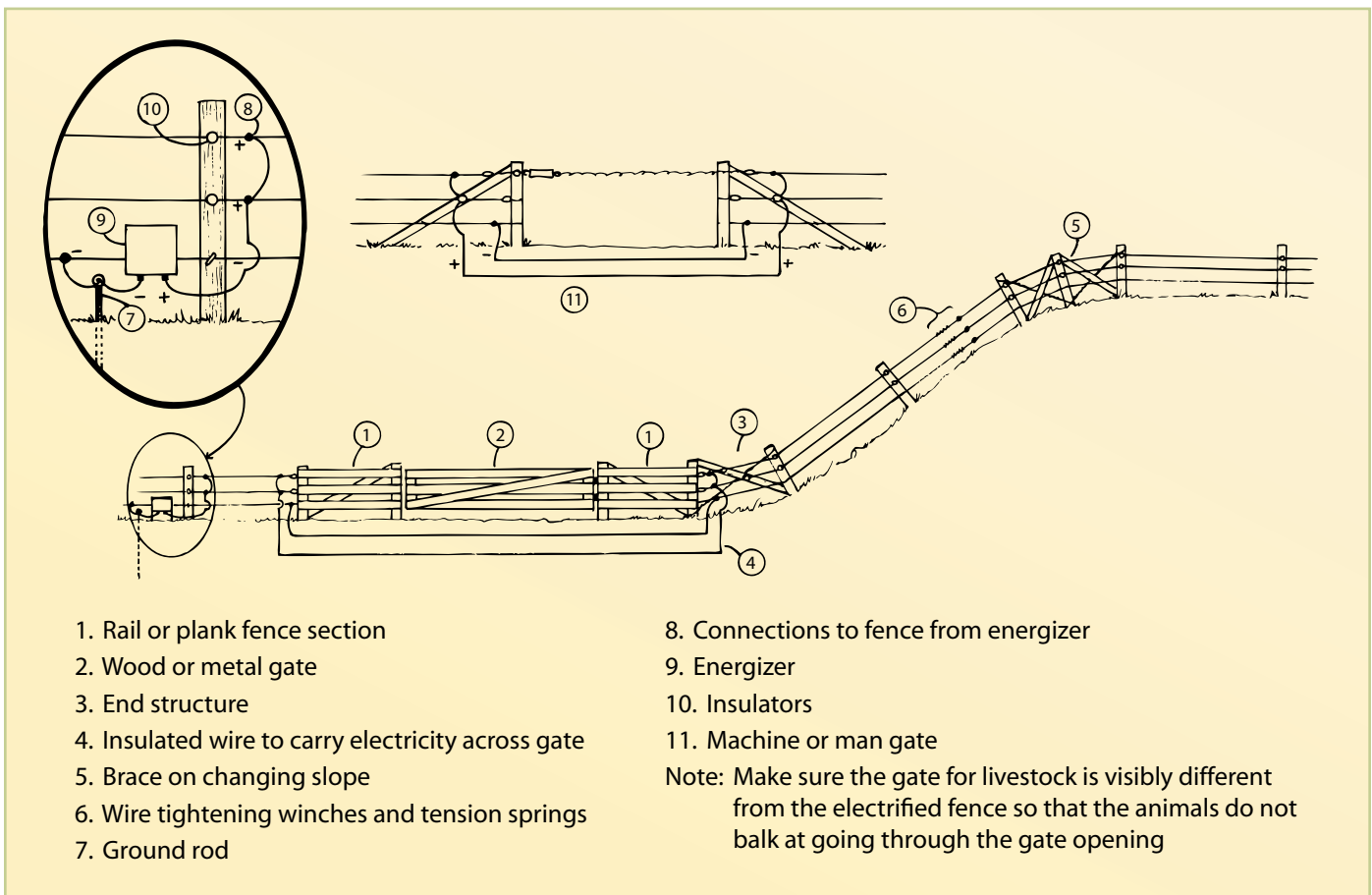
FIGURE 88. Permanent electric fence
