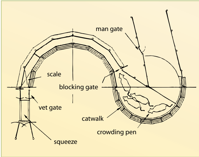
FIGURE 77. Working area combination – option two
