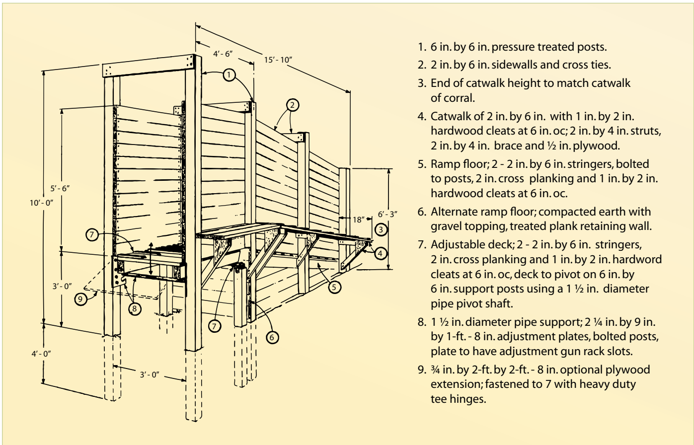
FIGURE 80. Loading chute design
