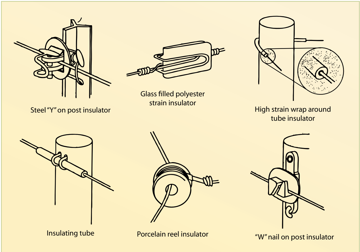
FIGURE 89. Types of insulators
