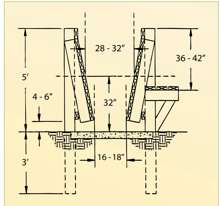
FIGURE 70. Fully tapered chute
