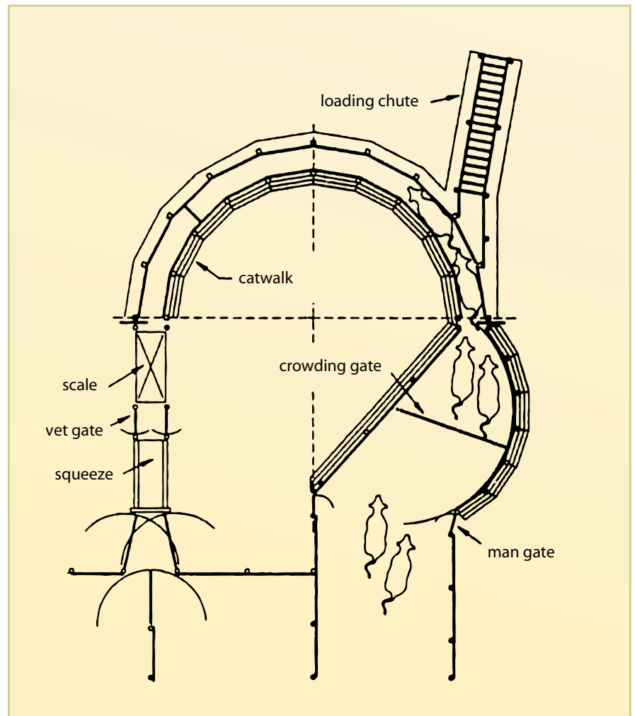
FIGURE 76. Working area combination – option one
