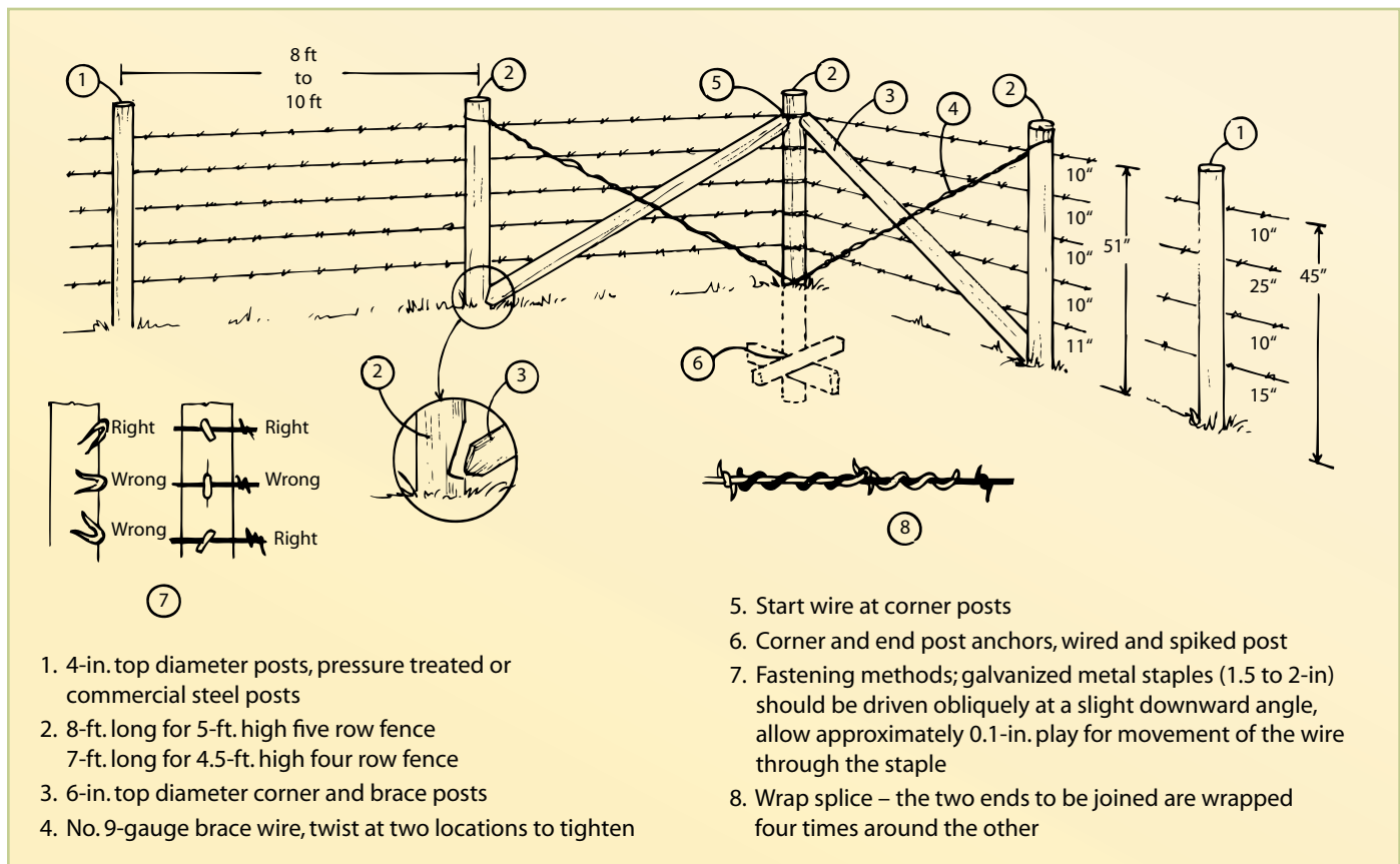
FIGURE 83. Barbed wire field fencing
