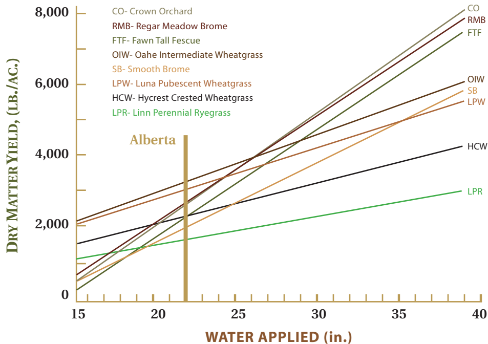
Figure 48. Water response functions for grasses (sunlight, temperature and nutrients not limiting)
