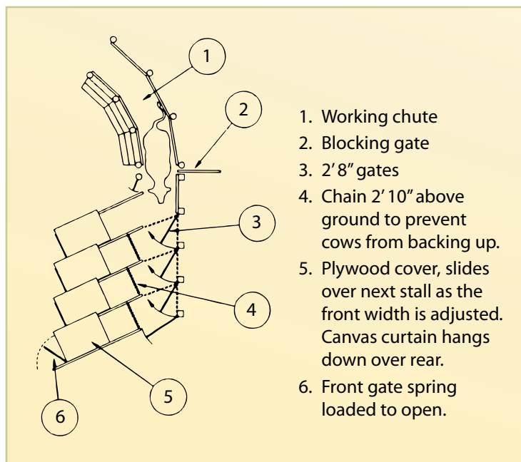
FIGURE 20. Herringbone AI breeding chute system
