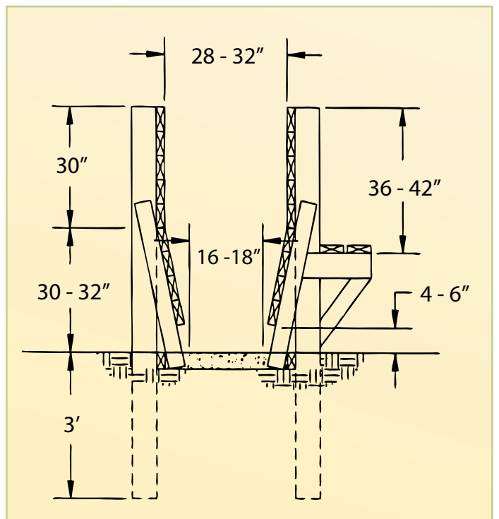
FIGURE 71. Half-tapered chute
