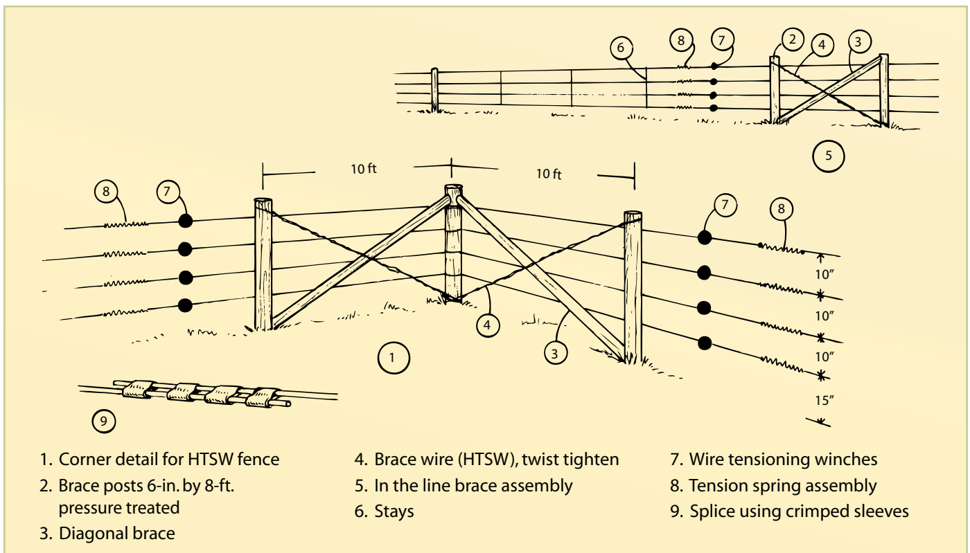
FIGURE 85. High-tensile smooth wire (HTSW) pasture fencing
