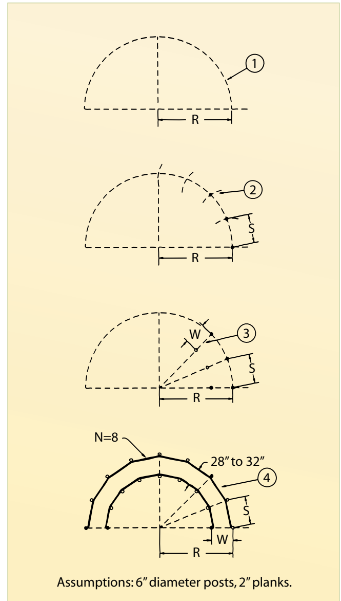
FIGURE 81. How to lay out a circular working chute
