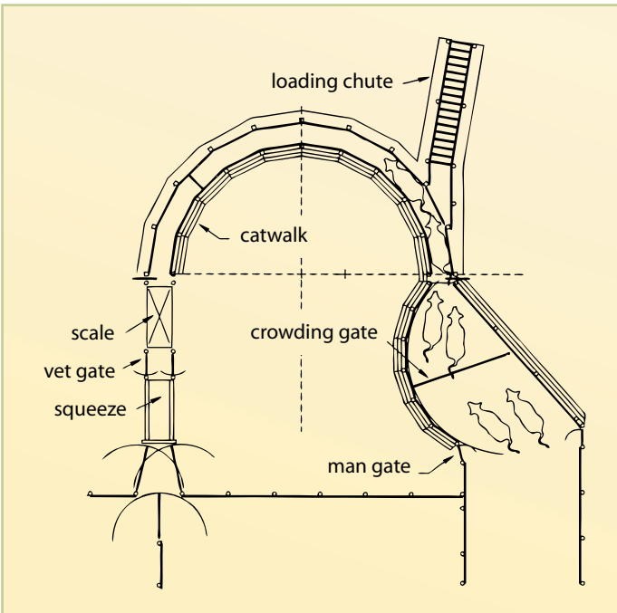
FIGURE 78. Working area combination – option three
