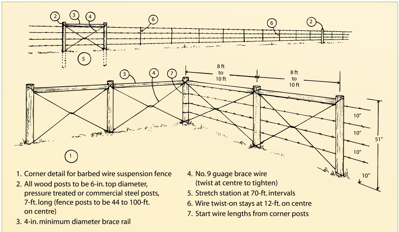
FIGURE 84. Barbed wire suspension fencing
